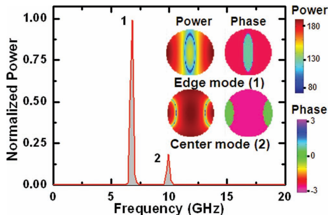
Figure 4. The power spectrum of the simulated magnetization dynamics of a single circular Py dot with 100-nm diameter and 20-nm thickness at H = 1.3\text{ kOe} . The power and phase maps of the two observed modes are shown in the inset. Mode 2 is identified as the centre mode while mode 1 as the edge mode of the Py dot.
