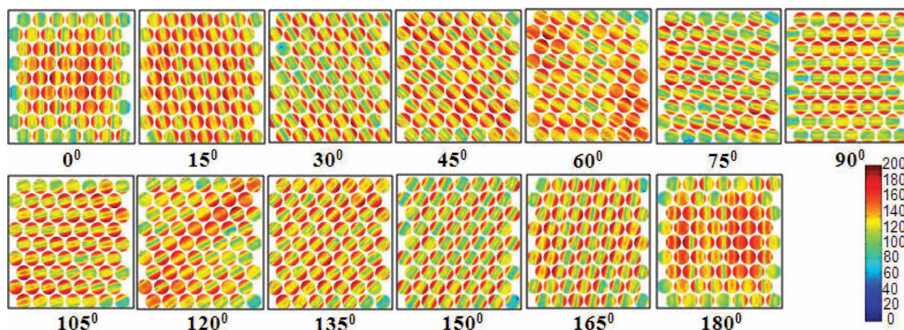
Figure 10. The power maps of mode 2 for the hexagonal lattice as a function of the azimuthal angle \phi of the in-plane bias magnetic field at H = 1.3 kOe. The variation of the overall power on the entire lattice structure with \phi indicates the variation of dynamic magnetization for this mode, which in turn gives the six-fold variation in the mode frequency.
