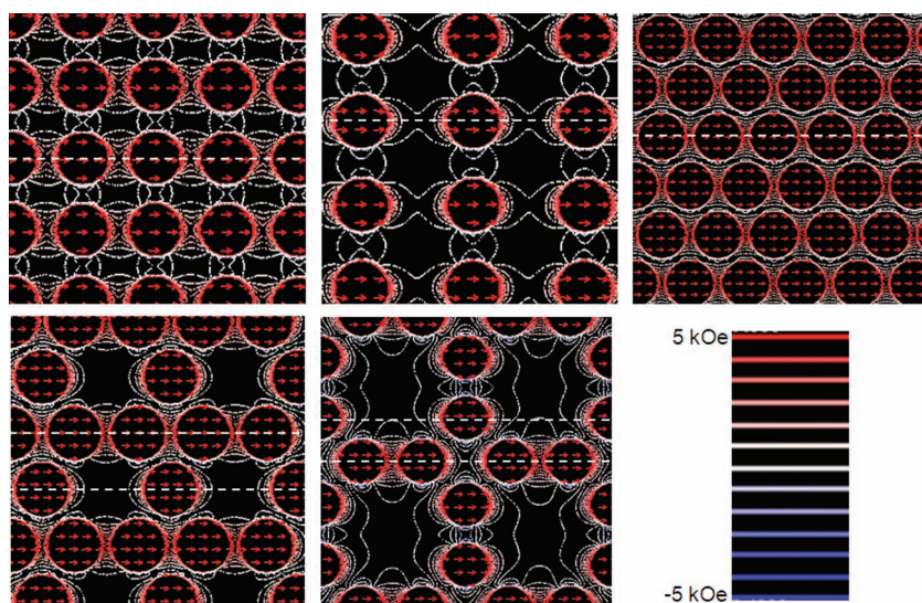
Figure 7. Contour maps of simulated magnetostatic field distributions (x-component) are shown for Py dots lattices with variable lattice symmetry at H = 1.3 kOe at \varphi = 0^\circ . The arrows inside the dots represent the magnetization states of the dots, while the strengths of the stray magnetic fields are represented by the color bar at the lower right corner of the figure. The horizontal dashed lines show the positions of the lattices, from which the linescans are presented in Figure 8.
